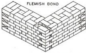
FLEMISH BOND
